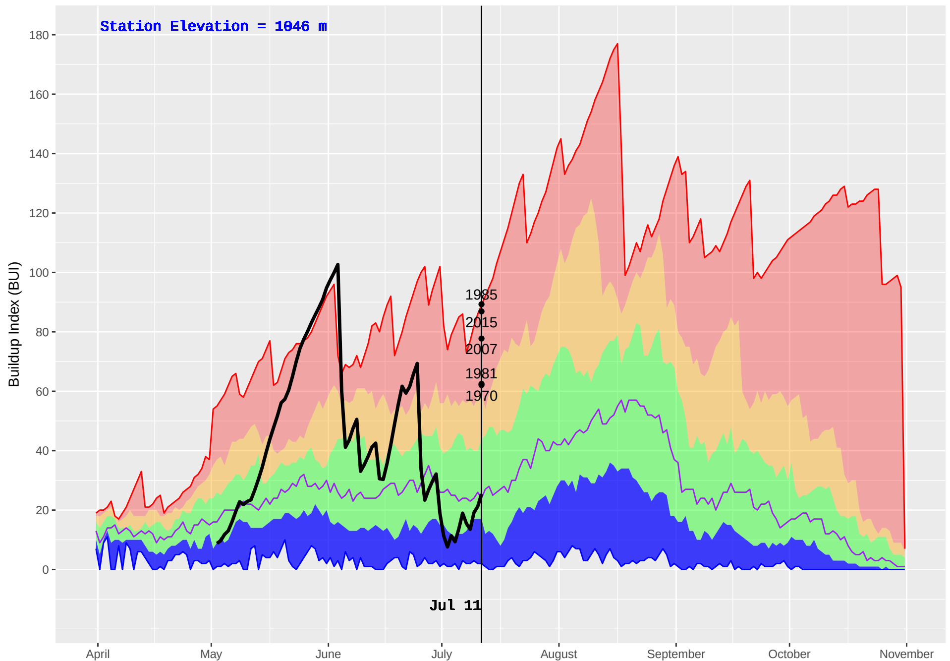
LIKELY RS (255) : Historical (1970–2016) and Current (2018) Noon Buildup Index (BUI)
