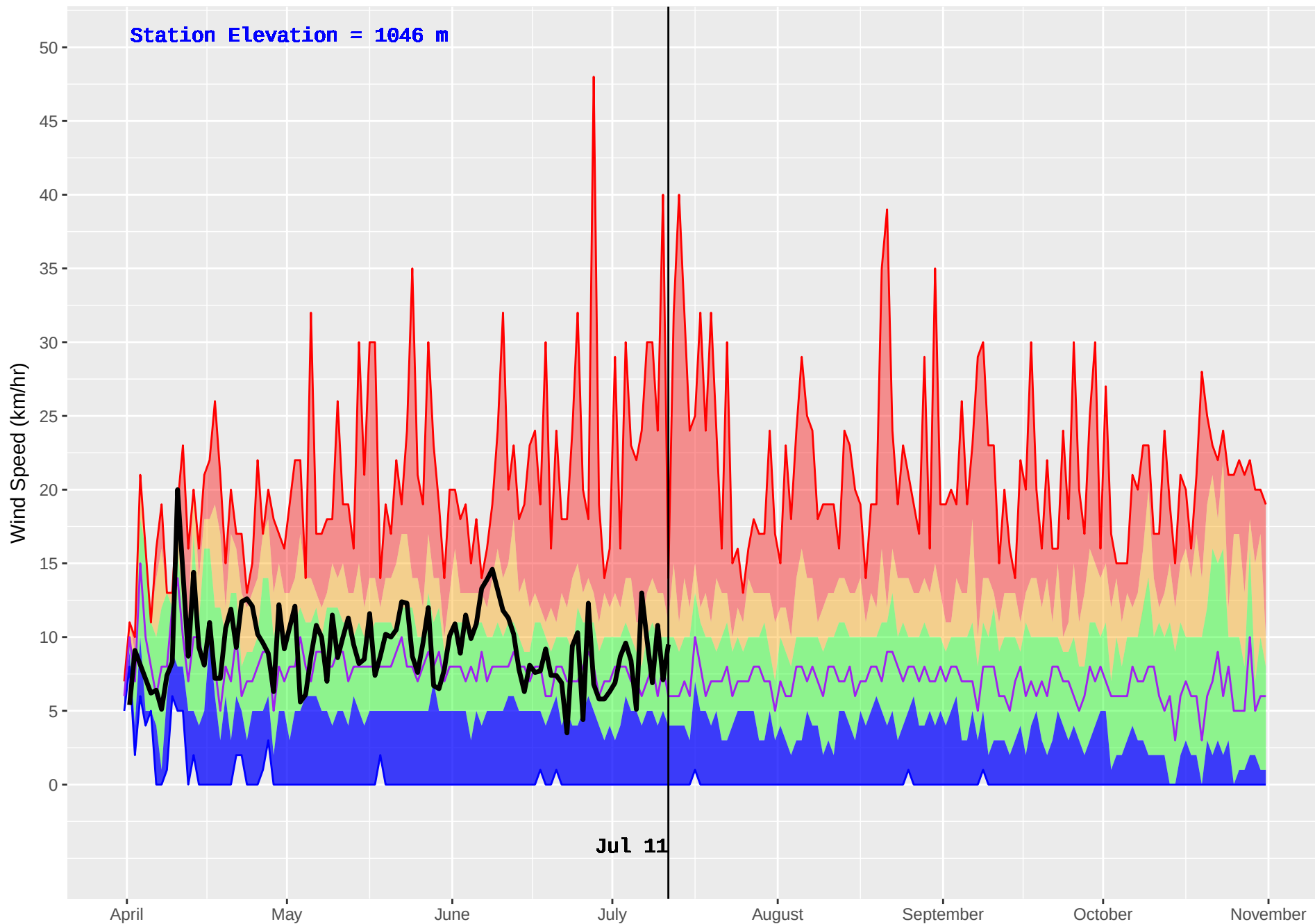
LIKELY RS (255) : Historical (1970–2016) and Current (2018) Noon Wind Speed
